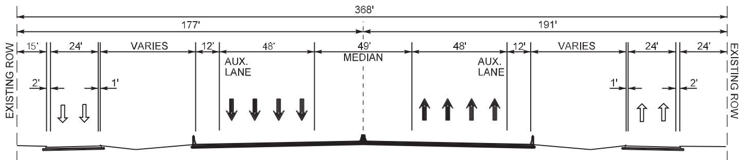
PROPOSED AT GRADE TYPICAL SECTION
