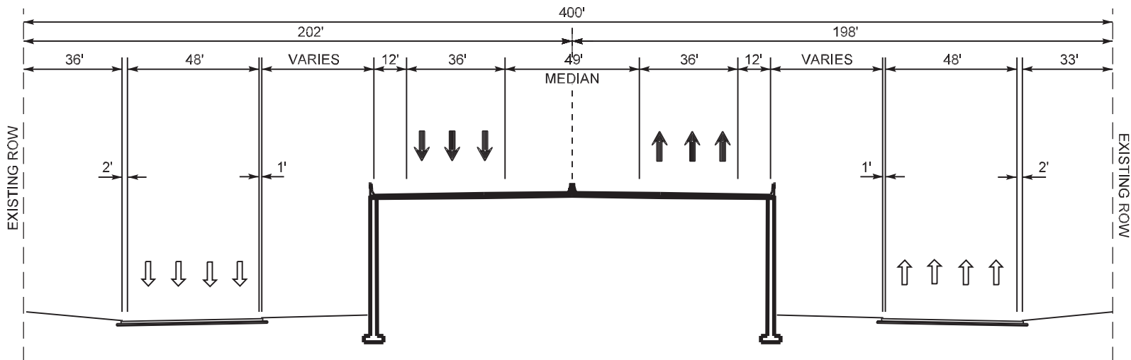
PROPOSED GRADE SEPARATED TYPICAL SECTION
