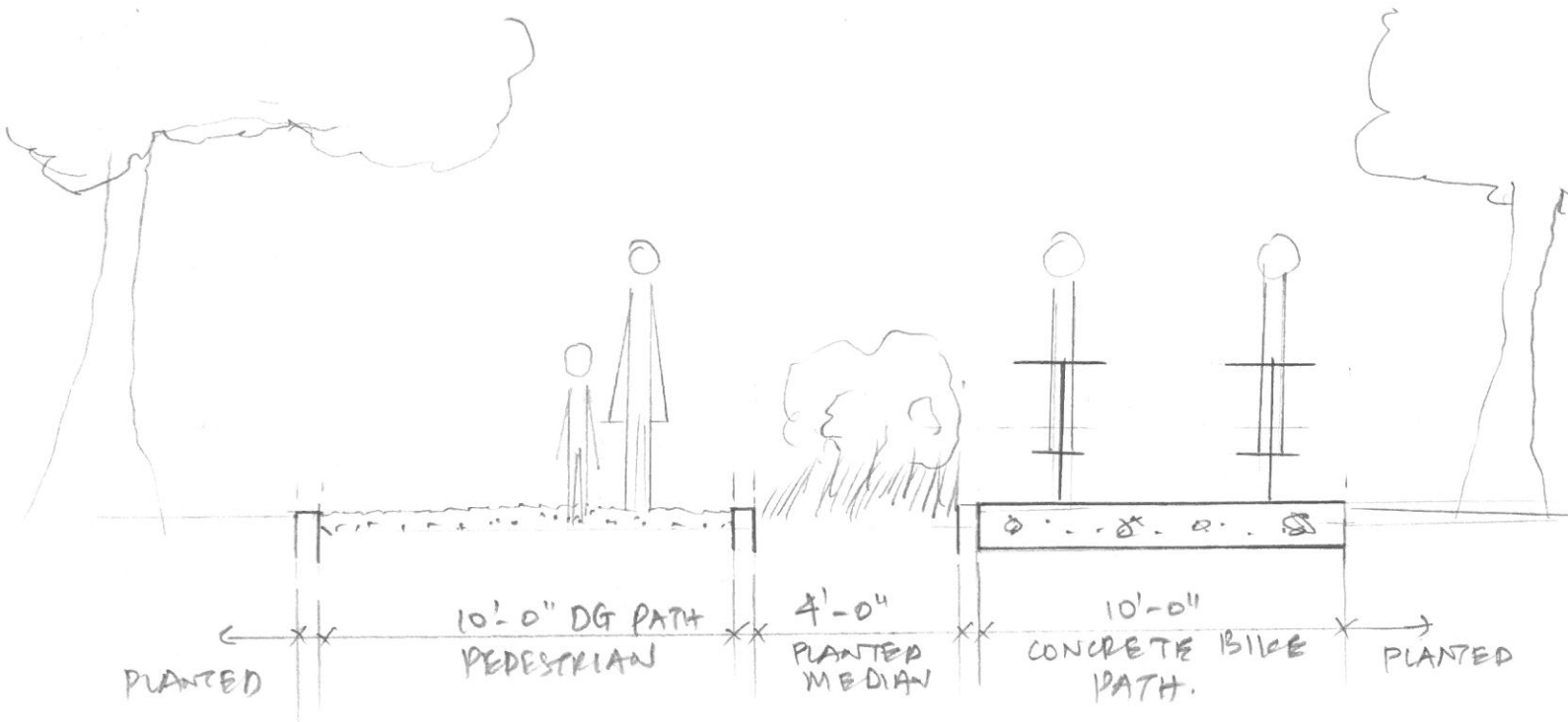
OFF STREET BIKE PATH SECTION
