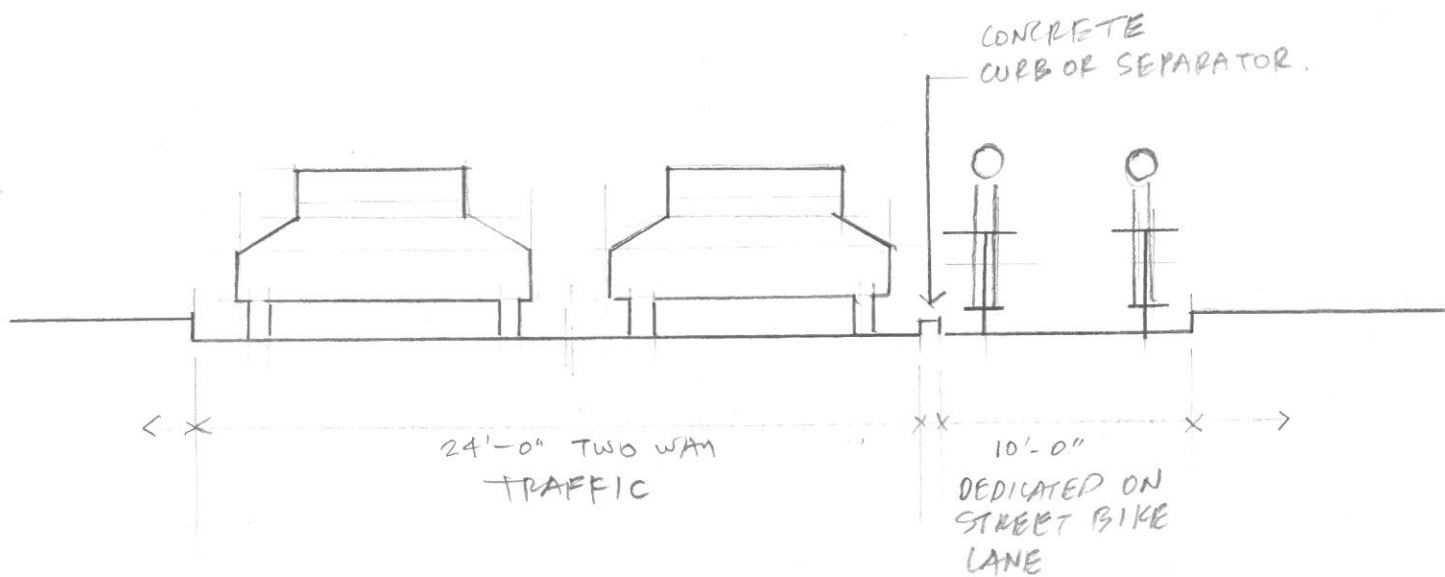
DEDICATED ON STREET BIKE PATH SECTION
