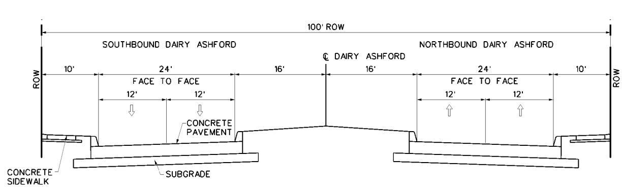
A EXISTING TYPICAL ROADWAY SECTION DAIRY ASHFORD ROAD FROM WESTHEIMER TO MEMORIAL N.T.S.
