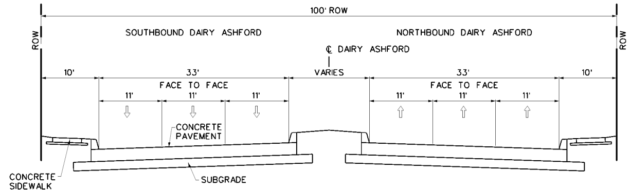
B EXISTING TYPICAL ROADWAY SECTION DAIRY ASHFORD ROAD FROM WESTHEIMER TO OVERBROOK FROM MEMORIAL TO I-10 N.T.S.
