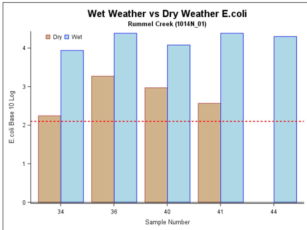
FIGURE 50. WET WEATHER AND DRY WEATHER E. coli CONCENTRATIONS FROM PHASE II RUMMEL CREEK SURVEYS. RED DOTTED LINE REPRESENTS THE STATE WATER QUALITY STANDARD FOR BACTERIA.
