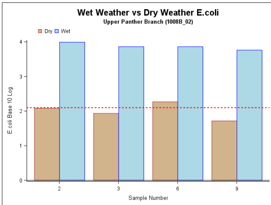
FIGURE 19. WET WEATHER AND DRY WEATHER E. COLI CONCENTRATIONS FROM PHASE II UPPER PANTHER BRANCH SURVEYS. RED DOTTED LINE REPRESENTS THE STATE WATER QUALITY STANDARD FOR BACTERIA.
