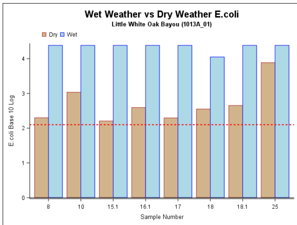
FIGURE 29. WET WEATHER AND DRY WEATHER E.coli CONCENTRATIONS FROM PHASE II LITTLE WHITE OAK BAYOU SURVEYS. RED DOTTED LINE REPRESENTS THE STATE WATER QUALITY STANDARD FOR BACTERIA.
