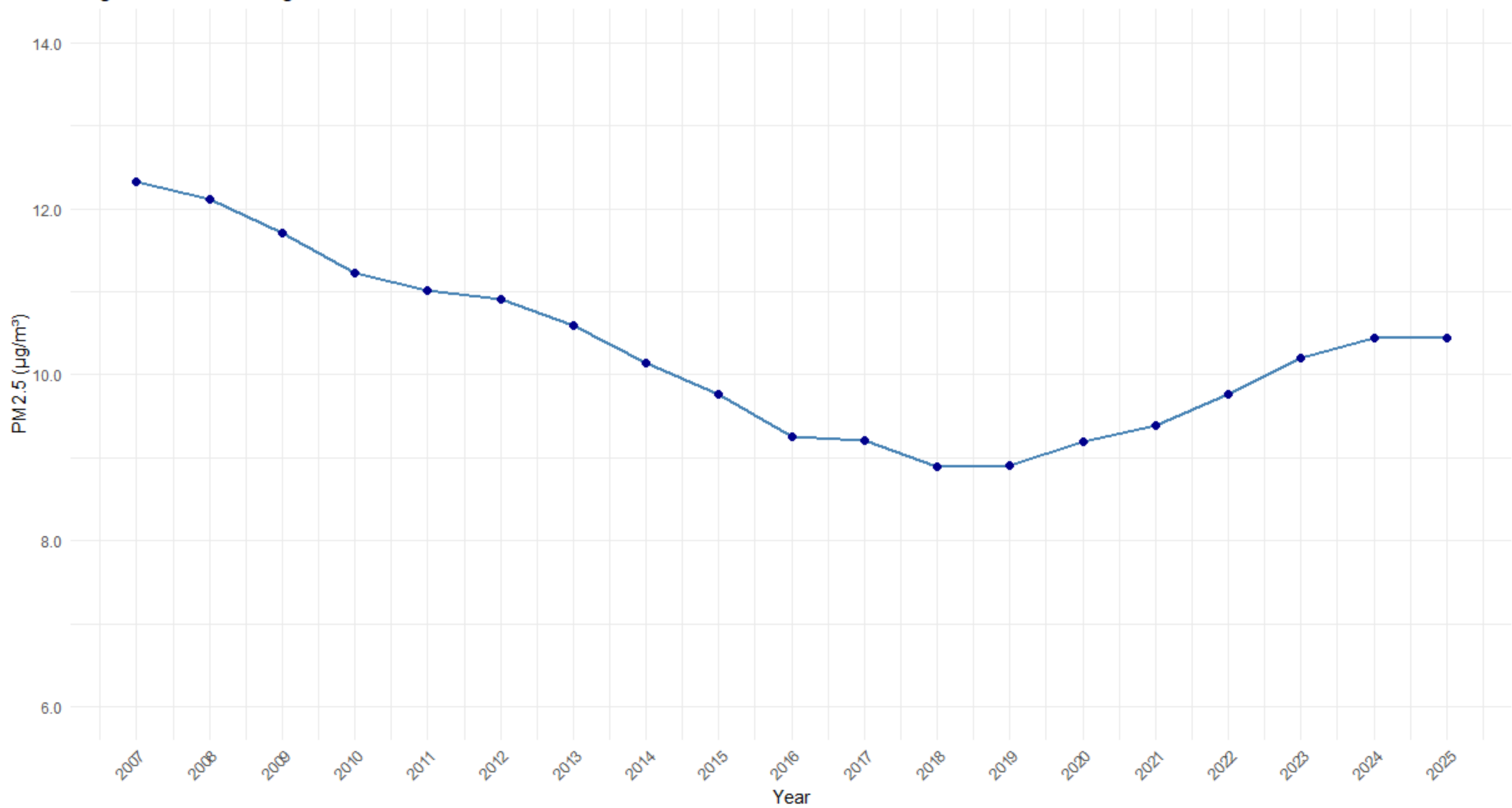
Regional PM2.5 Design Value, 2007-2025
