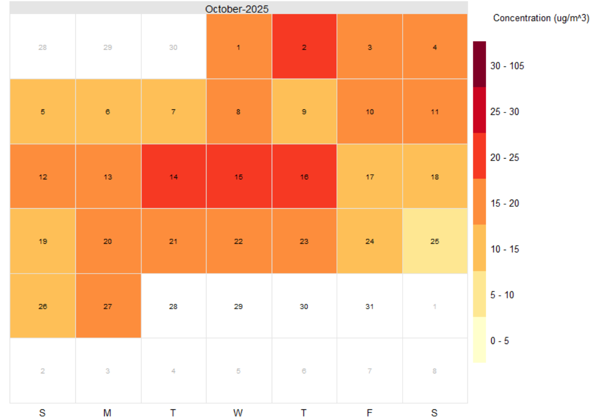
Daily Max PM 2.5 Concentration (Baytown, October 2025)
