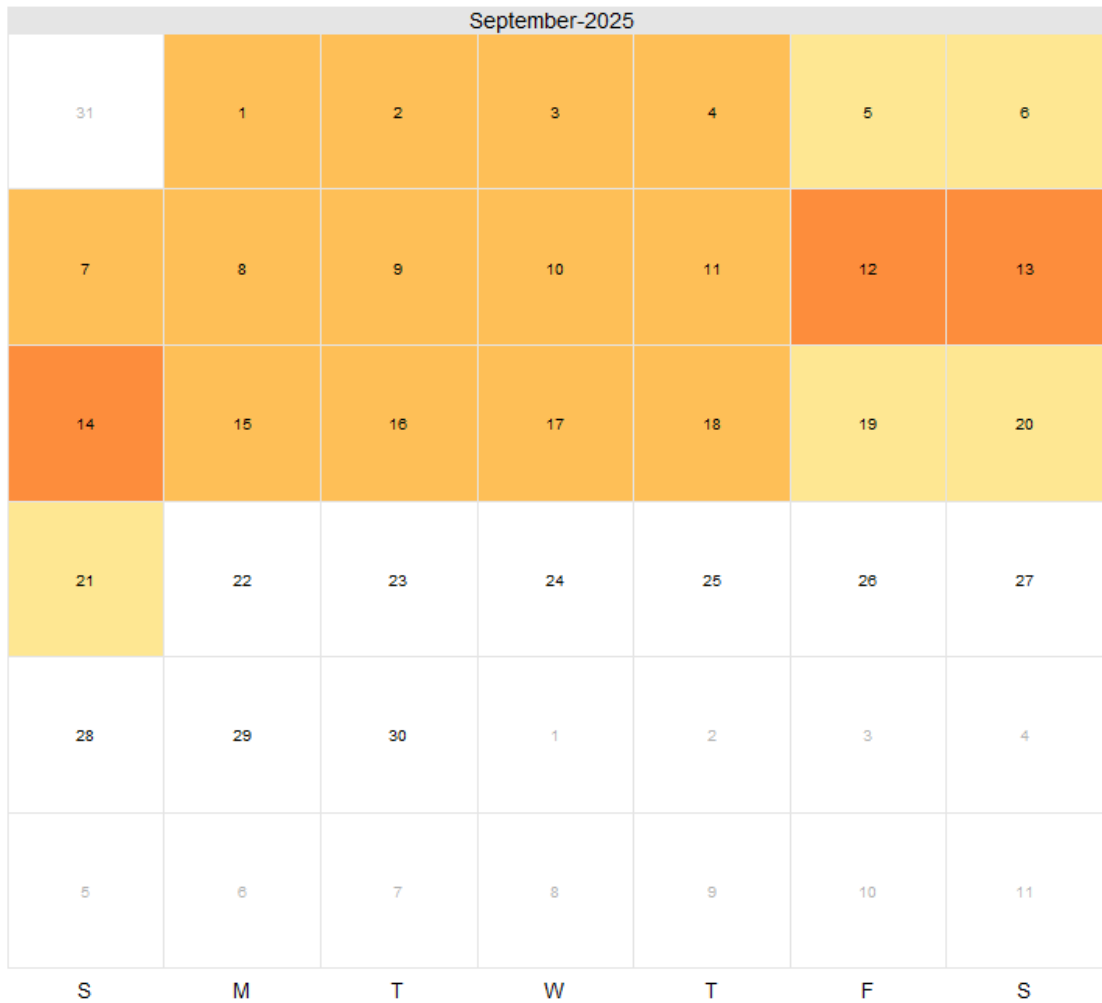
Mean Daily Mean PM 2.5 Concentration (All Monitors, September 2025)
