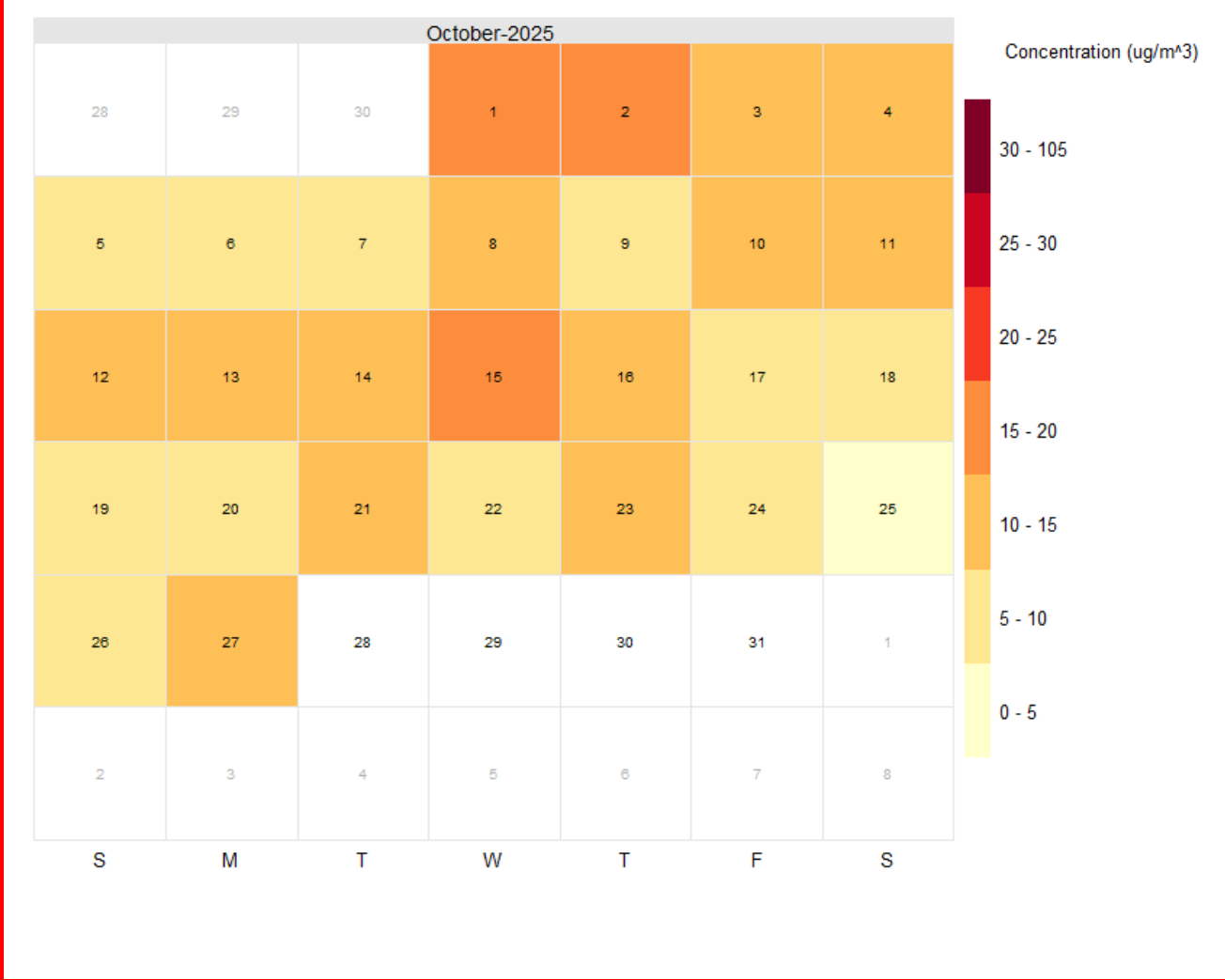
Mean Daily Mean PM 2.5 Concentration (All Monitors, October 2025)
