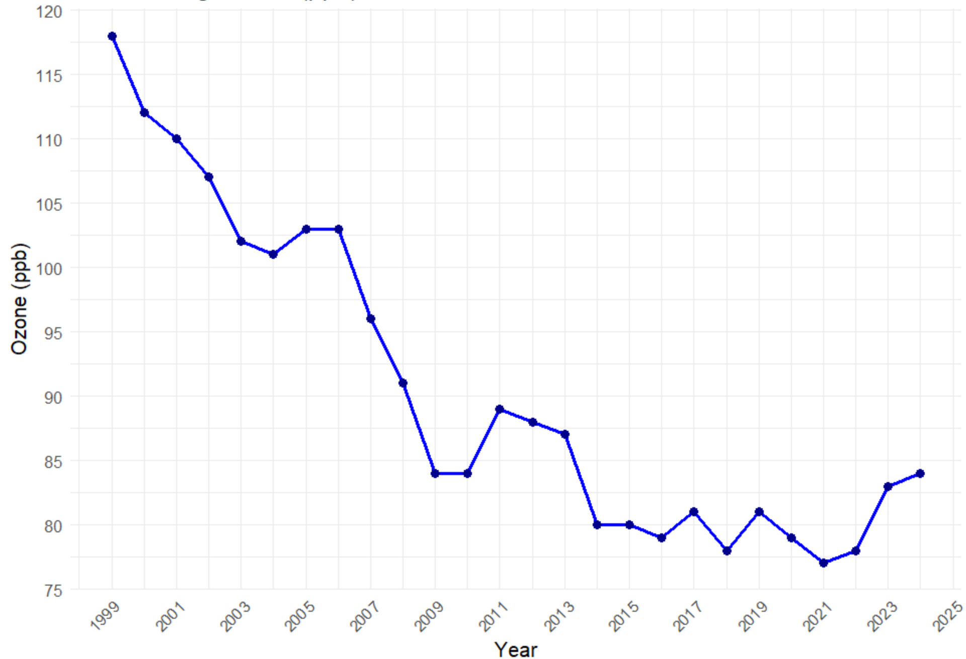
Ozone Design Value (ppb), 1999-2024
