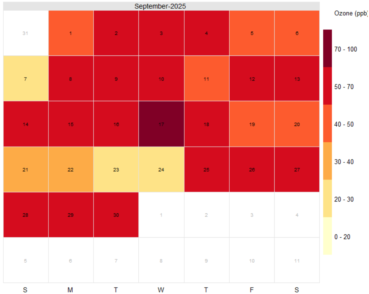
Mean Daily Maximum 8-Hour Ozone Concentration (All Monitors, September 2025)
