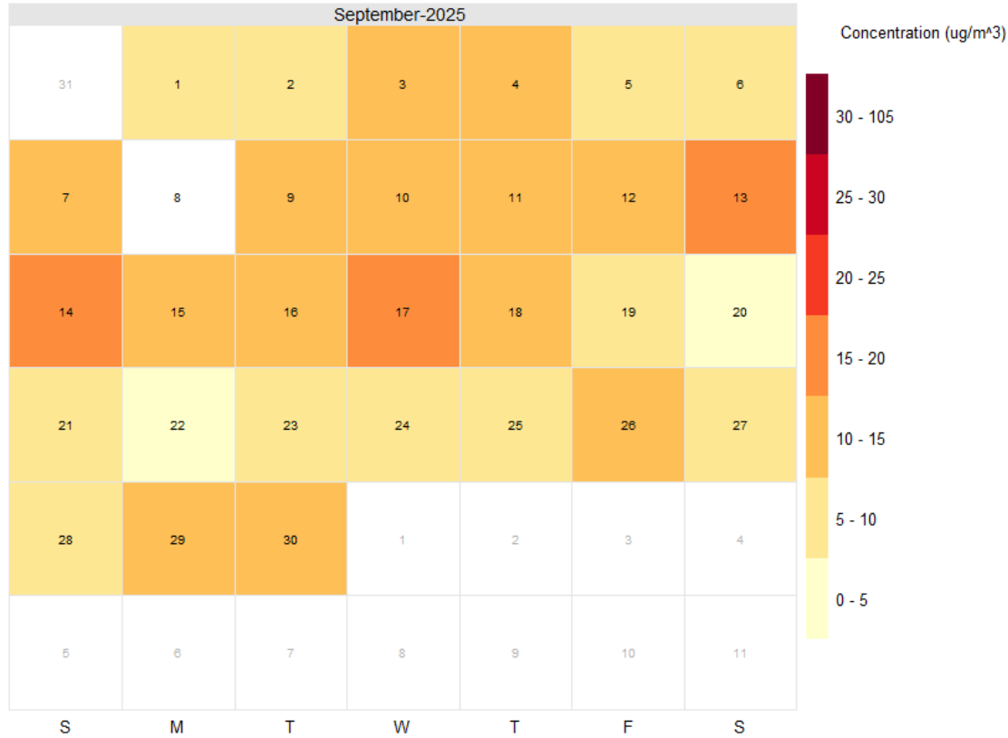
Daily Max PM 2.5 Concentration (Baytown, September 2025)
