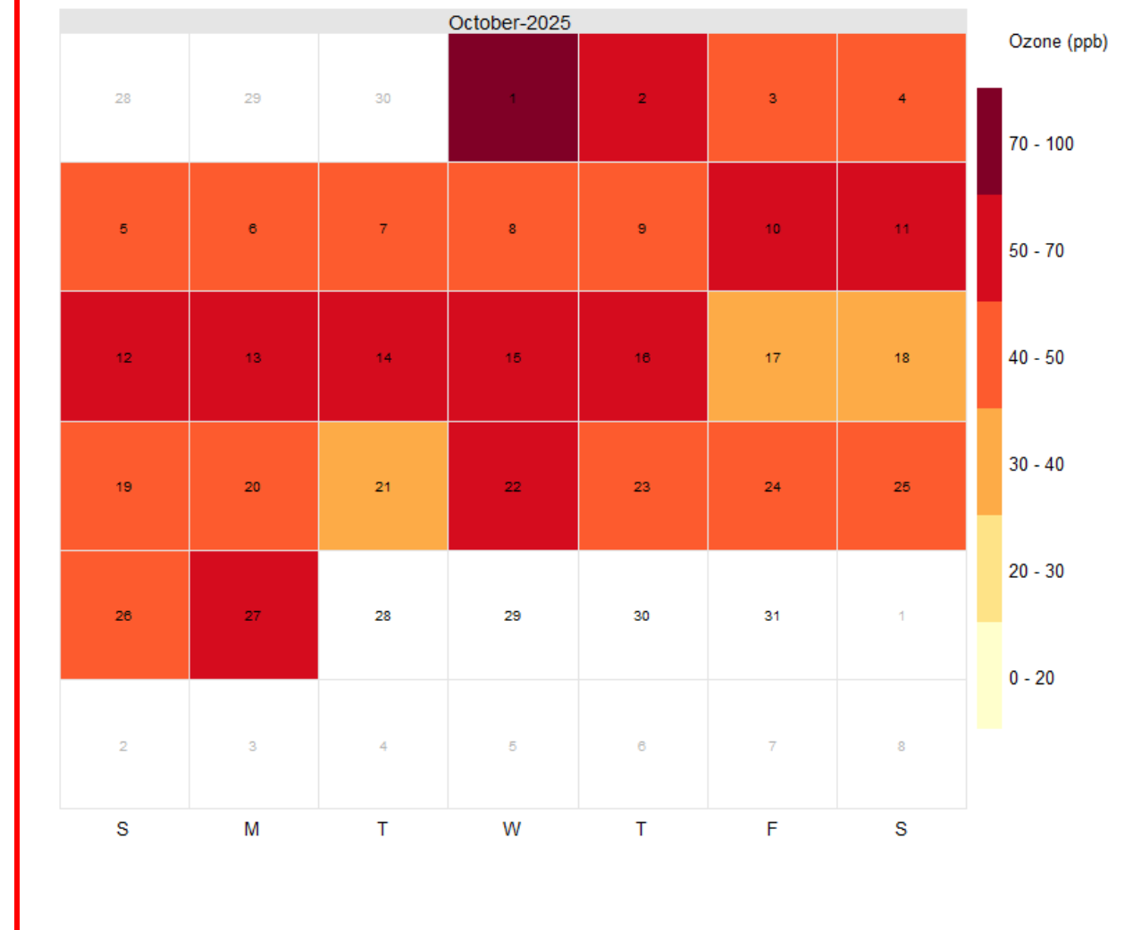
Mean Daily Maximum 8-Hour Ozone Concentration (All Monitors, October 2025)
