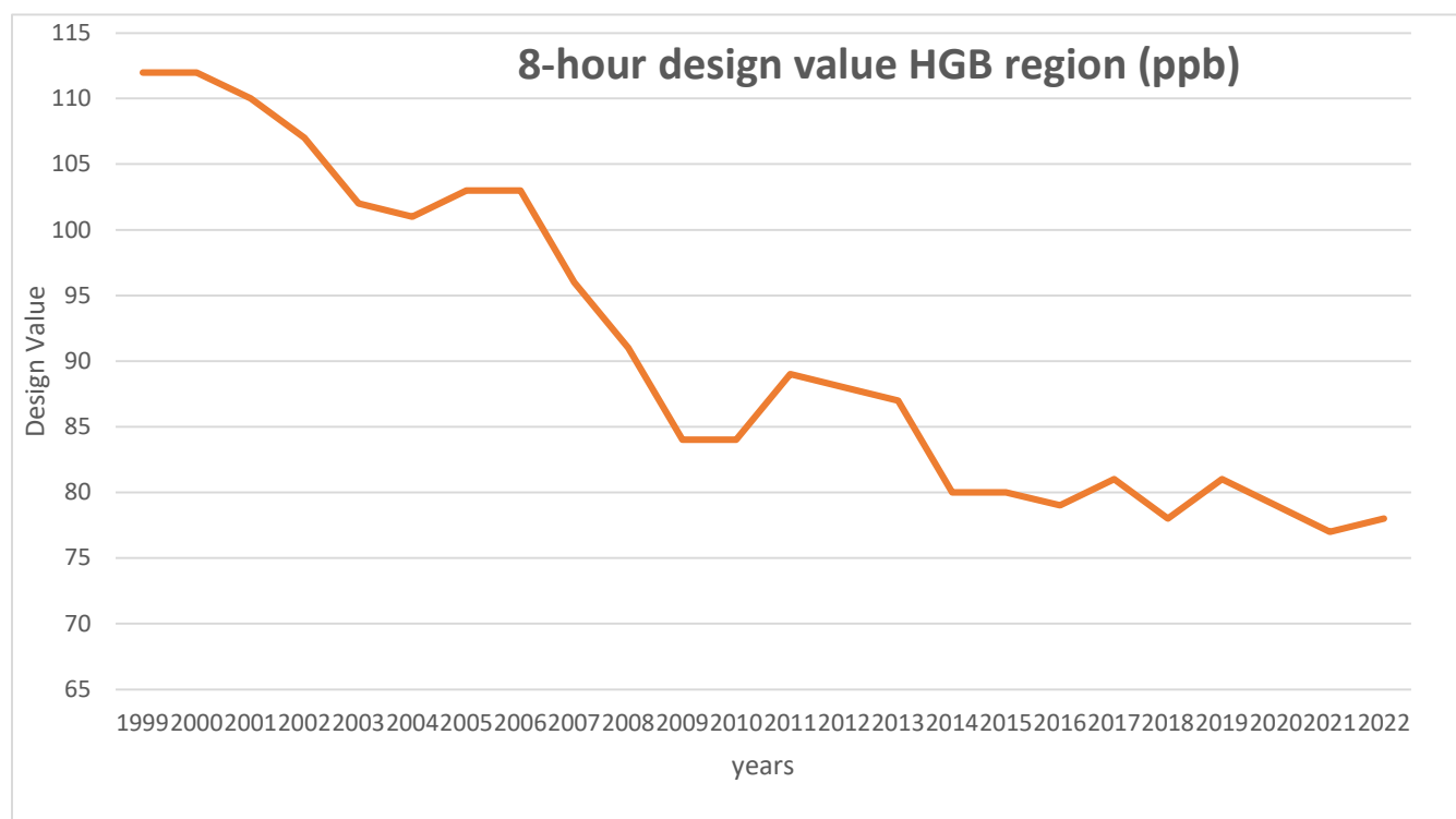
Figure 2.1 8-hour Ozone Design Values (in ppb)
