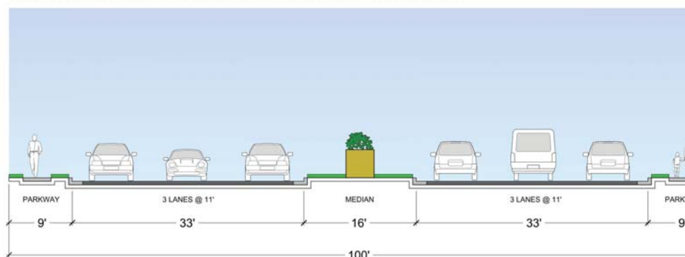
Figure 3.2: Typical section details for corridor
