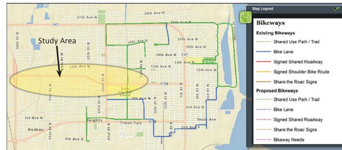
Figure 3.9: H-GAC Regional Bikeway Plan, June 2010, showing no current or planned bicycle facilities along the study corridor. A trail crosses the corridor at the signal for the school and library.
