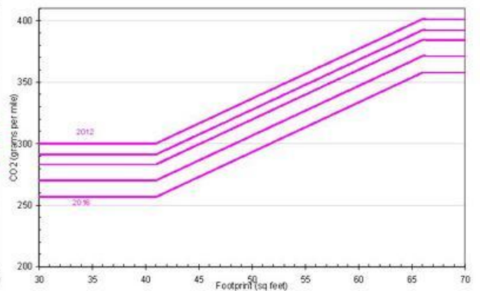
Figure 2 - CO 2 (g/mi) Truck Standard Curves
