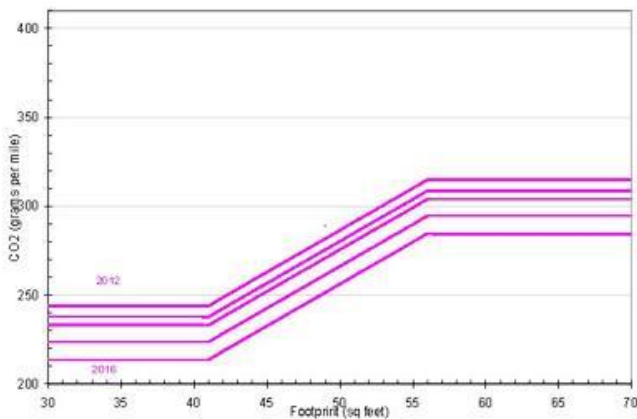
Figure 1 - CO 2 (g/mi) Car Standard Curves
