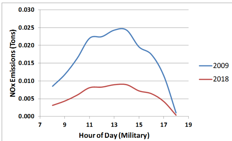
Figure 11. Heavy-Duty Truck NOx Emissions, Bayport Terminal
